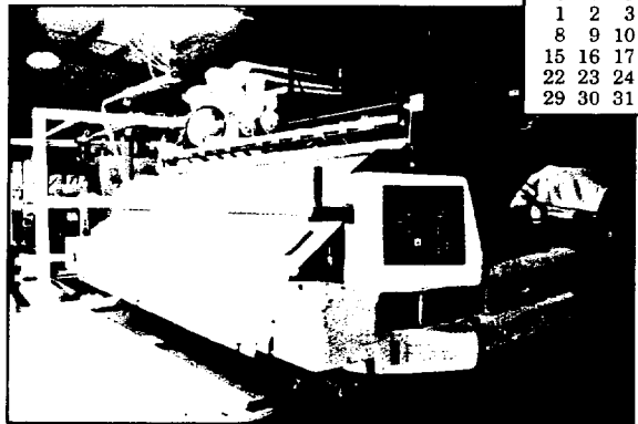
Cloth Spreading Machine
